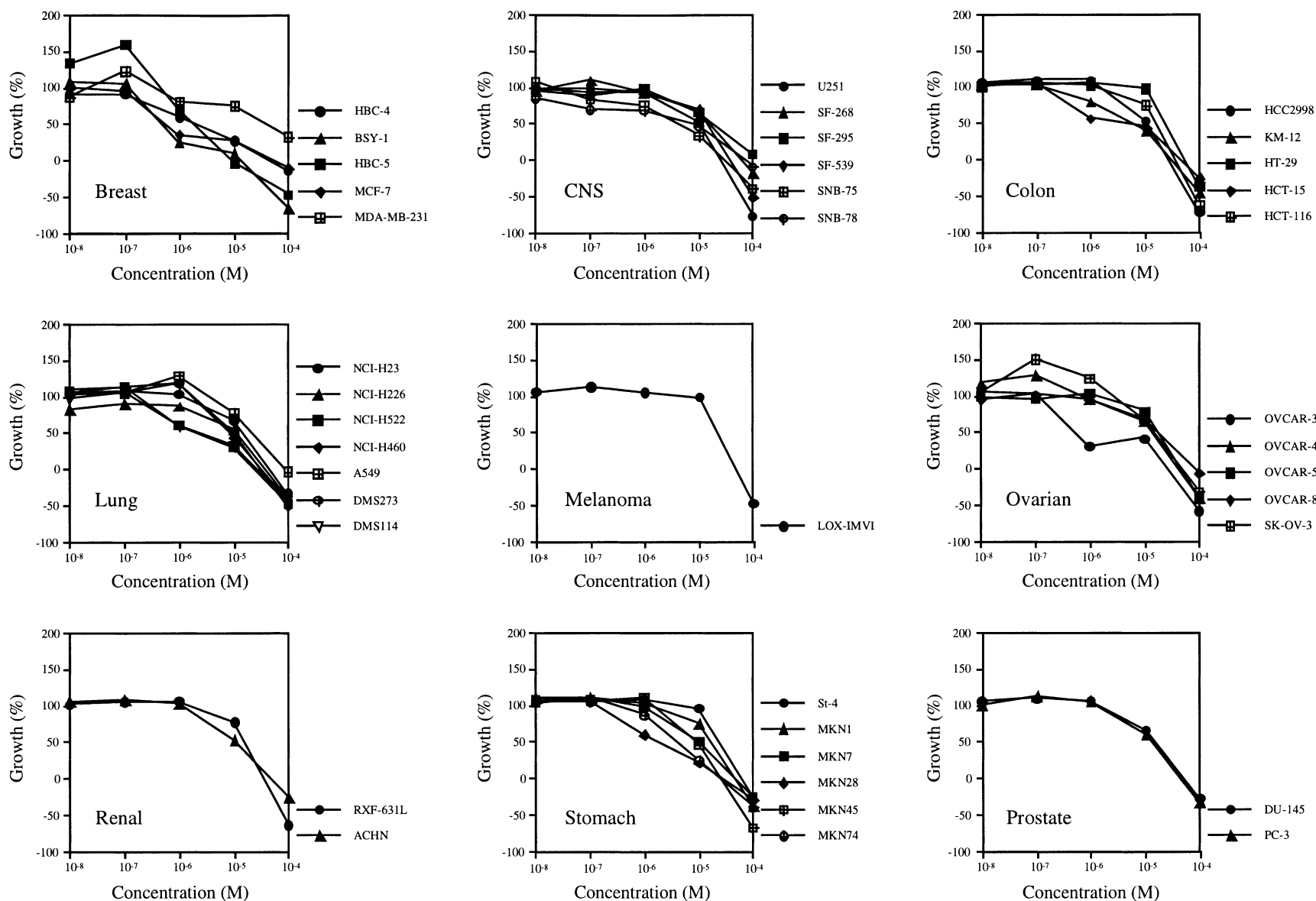
Figure 1. Dose-response curves of compound 7 on HCC panel. Test compound concentration; 10^{-4} – 10^{-8} M.
