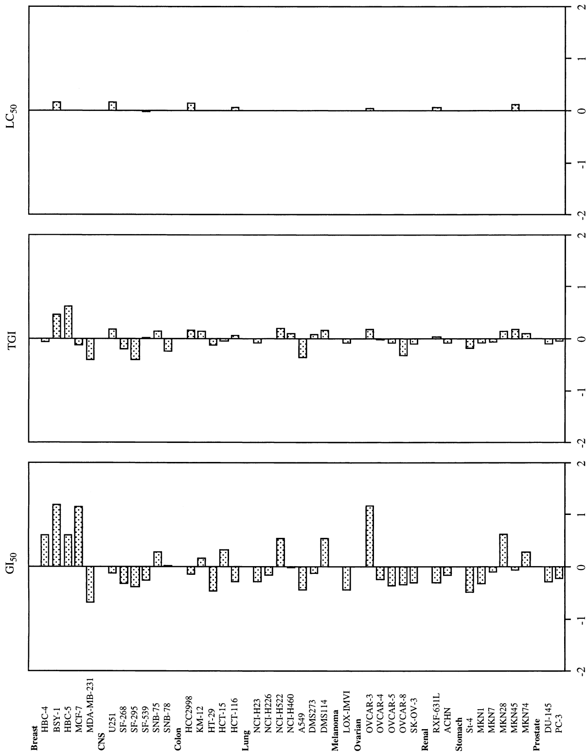
Figure 2. Mean graph of compound 7 on HCC panel.
